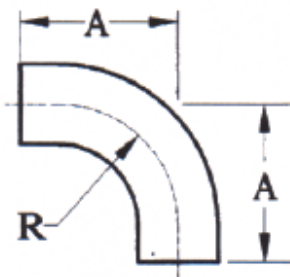
3D 90 Degree Plain Bend R=3xd
