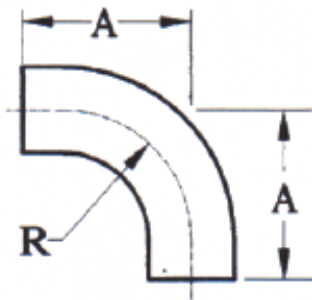
2D 90 degree Plain Bend R=2xd
